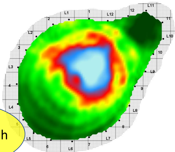
Improved detail using Ludwig Sensors
